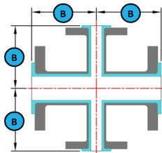
Reducing Cross
