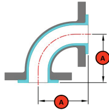
90 Degree Elbow
