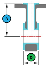
Instrument Tee
