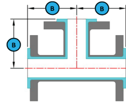
Equal Tee
